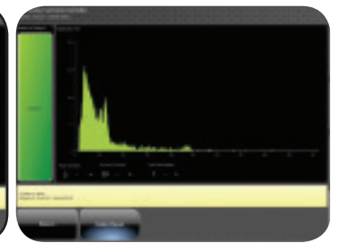
Barium-133 Spectra
